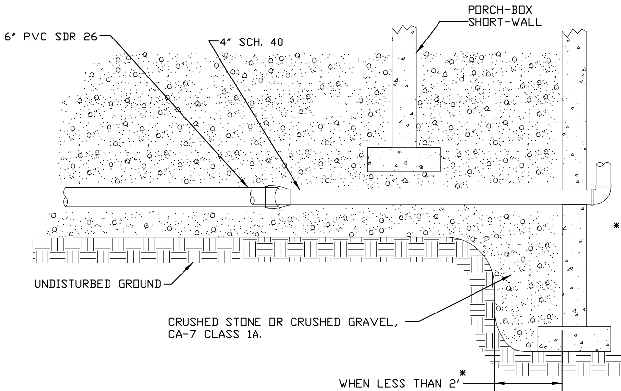
TYPICAL DETAIL FOR SANITARY SERVICE UNDER PORCH BOX FOOTING
